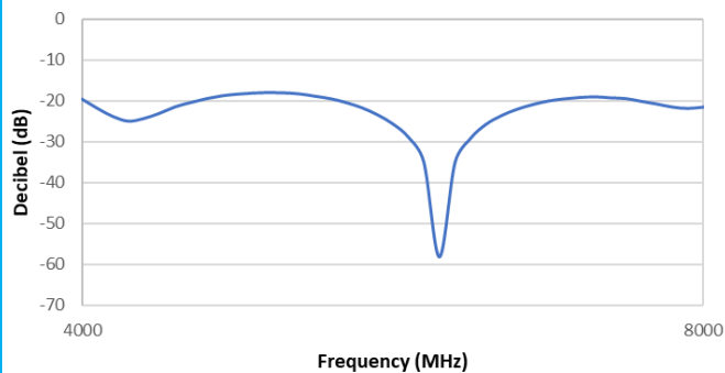
Isolation (dB)
