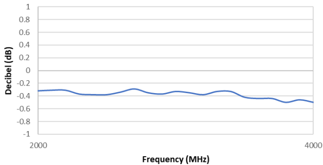
Insertion Loss (dB)
