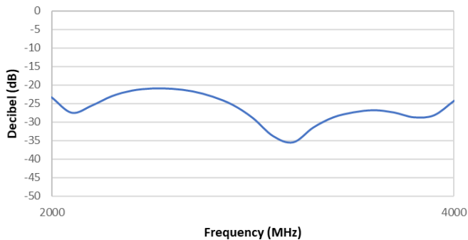
Isolation (dB)
