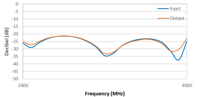
Return Loss (dB)
